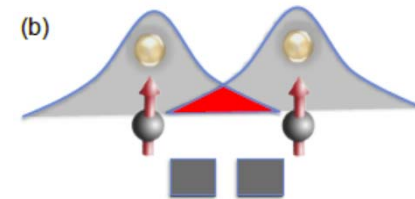
Interaction between two Shiba states: Yao et al., 13092633
