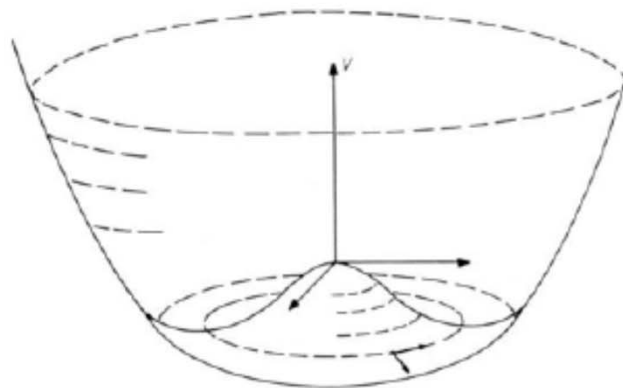
Bogoliubov qp
