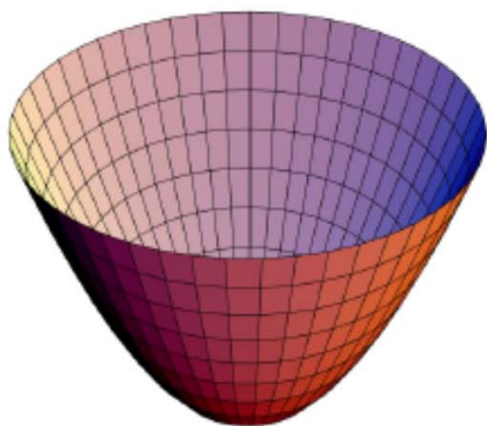
impurity
