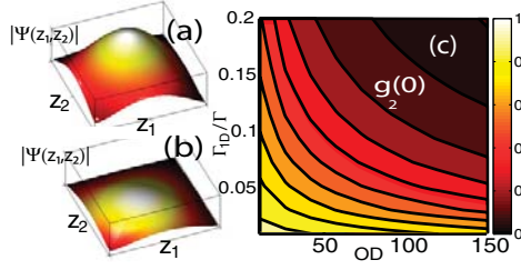
Fig. 4: (Colour on-line) Nonlinear absorption: two-photon wave function amplitude in the absence ( \Delta_2 \gg \Gamma ) (a) and presence ( \Delta_2 = 0 ) (b) of nonlinear absorption. The physical parameters are chosen such that OD = 70 , T \simeq 20\% and \frac{\Gamma_{1D}}{\Gamma} = 10\% . (c) Correlation function g_2(\tau = 0) of the transmitted light as a function of optical depth (OD) and single-atom cooperativity when the frequency is set to the single-photon transmission resonance with T \simeq 20\% and \frac{\Delta_2}{\Gamma} = 0 .
