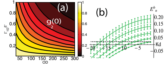
Fig. 3: (Colour on-line) (a) Repulsive photons: correlation function g_2(\tau=0) of the transmitted light as a function of optical depth ( OD = n_0 L \frac{\gamma_0}{\Gamma} ) and single-atom cooperativity when the frequency is set to the single-photon transmission resonance with T \simeq 20\% and \frac{\Delta_2}{\Gamma} = 5 . (b) Attractive photons: bound state energies (solid) become resonant with energies of incoming photons (dashed) for specific values of \kappa . The error bars represent the decay rate of each bound state.
