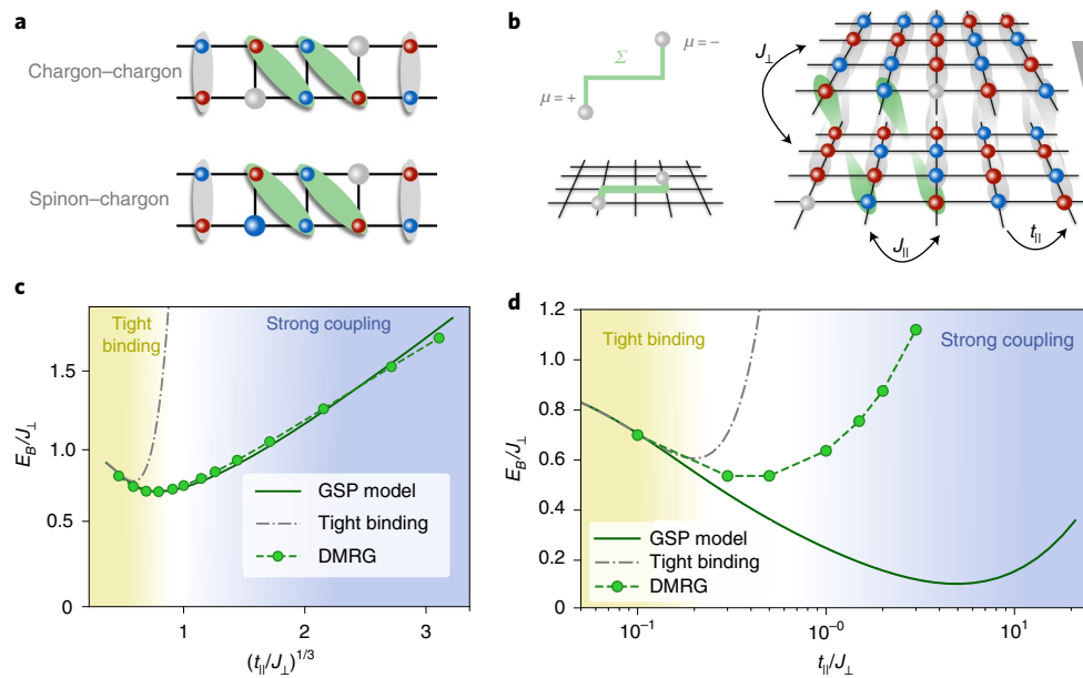
Fig. 1 | String-based chargin pairing in mixD bilayers. We introduce an efficient pairing mechanism for distinguishable chargeons with flavours \mu = \pm connected by a string \Sigma . a,b , The string pairing mechanism can be realized in a model of d -dimensional bilayers with spin-1/2 particles and strong repulsive interactions for d=1 ( a ) and d=2 ( b ). We consider mixD systems, where the hopping t_{\perp} between the layers is suppressed by a gradient \Delta , while the superexchange J_{\perp} is kept intact and J_{\perp} \gg J_{\parallel} . The strong interlayer superexchange leads to the formation of rung singlets (dimers indicated by grey ellipses with red and blue spheres), depicted here for d=1 ( a ) and d=2 ( b ). The motion of doped holes (grey spheres) via t_{\parallel} within different layers \mu = \pm tilts the singlets along their paths, which corresponds to the formation of \Sigma . The potential energy associated with the string increases with its length as more singlets are tilted. Grey (green) shading corresponds to vertical (tilted) singlets. c,d , E_B obtained by comparing the energies of spinon-chargeon and chargeon-chargeon mesons in the GSP model, and the ground-state energy for a system with one versus two holes in DMRG as described in the text. We assumed that J_{\parallel}/J_{\perp} = 0.01 and varies t_{\parallel}/J_{\perp} in equation (4). In the DMRG, weak interlayer tunnelling of strength t_{\perp}/J_{\perp} = 0.01 was added to ensure convergence. The shading indicates the tight binding and strong coupling regimes. c , E_B for a 40 \times 2 ladder ( d=1 ). d , E_B for a bilayer system on a 12 \times 4 cylinder.
